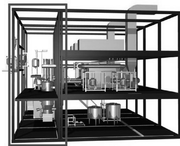
Fig. 2. Modular construction of a pharmaceutical facility. The frames indicate the steel modules used to assemble the facility (reproduced with kind permission of Pharmadule, Sweden).
