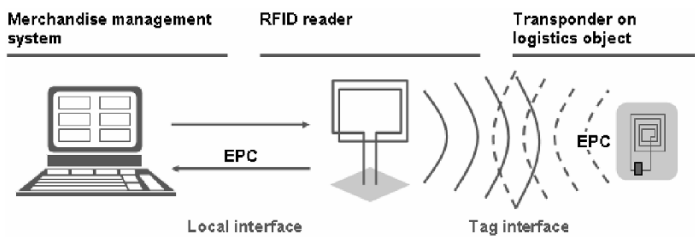
Fig. 9. RFID identification
