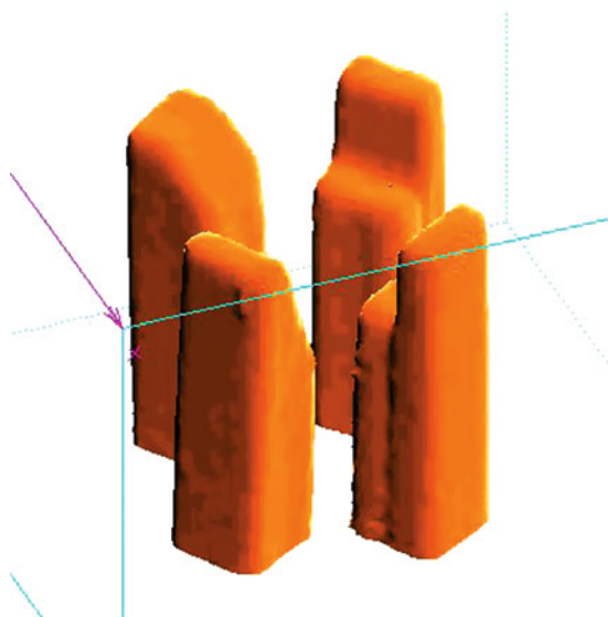
Fig. 10.11 Optical CT of four irradiations of the CCO beam (8 Gy at full modulation) in a PRESAGE TM polymer. The beam direction is from below, and demonstrates the effect of two wedges ( left ) and two “Al-blocked fields” ( right ). With kind permission of S. Doran, ICR UK
