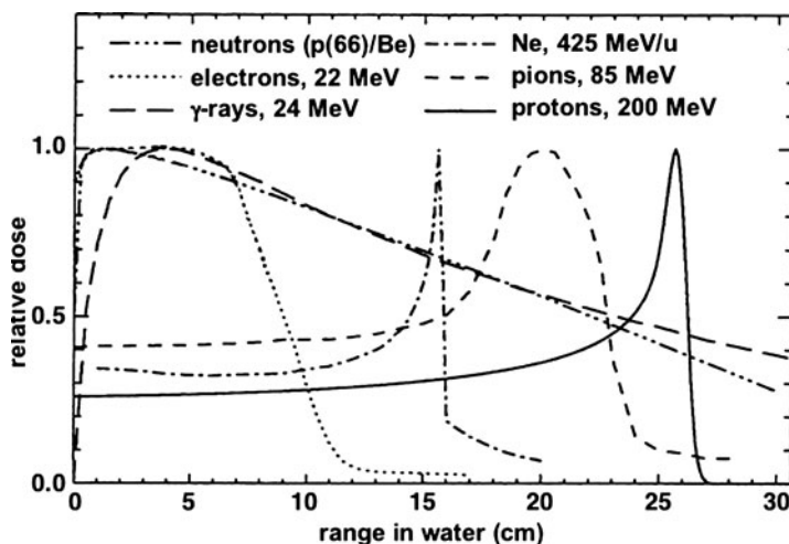
Fig. 4.2 Depth-dose distributions of various kinds of radiation in water
