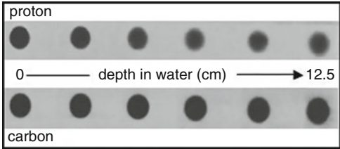
Fig. 4.4 Multiple scattering in a narrow ion beam ( \varnothing 9 mm). Comparison of protons and carbon ions. The higher angular deflection of the particles in the proton beam leads to a visible loss of particle density in the proton spots. Spotsize and particle density of the carbon beam change only slightly. Data from GSI, Darmstadt
