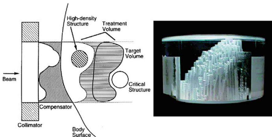
Fig. 25.12 Representation ( left ) of how a compensator ( right ) is used to account for density variations in the target and allow for conformity to the distal edge despite a fixed distal range of the beam
