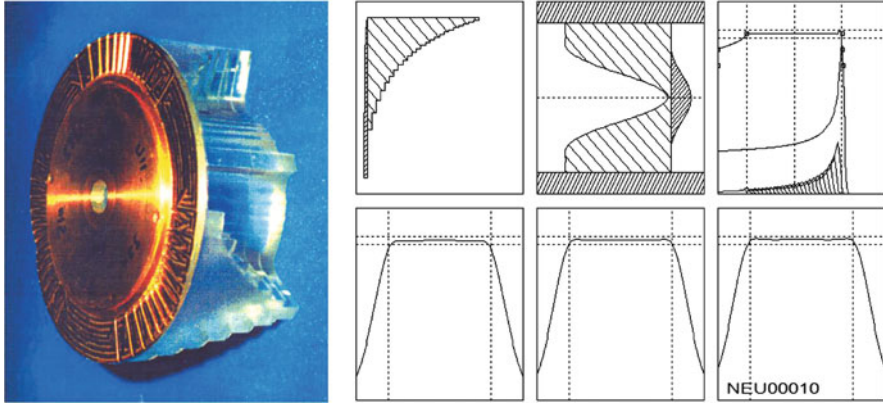
Fig. 25.15 An example of a scattering power-compensated range modulator ( left ), and a calculation including the use of a contoured scatterer ( right: upper middle graph ), as part of a calculation to optimize a double scattering system using NEU [3]. The graphs to the right (from Bernard Gottschalk) include the thickness of the range modulator wheel ( upper left ), the resulting Bragg peak distribution ( upper right ), and the transverse distributions at three depth locations ( lower three graphs )
