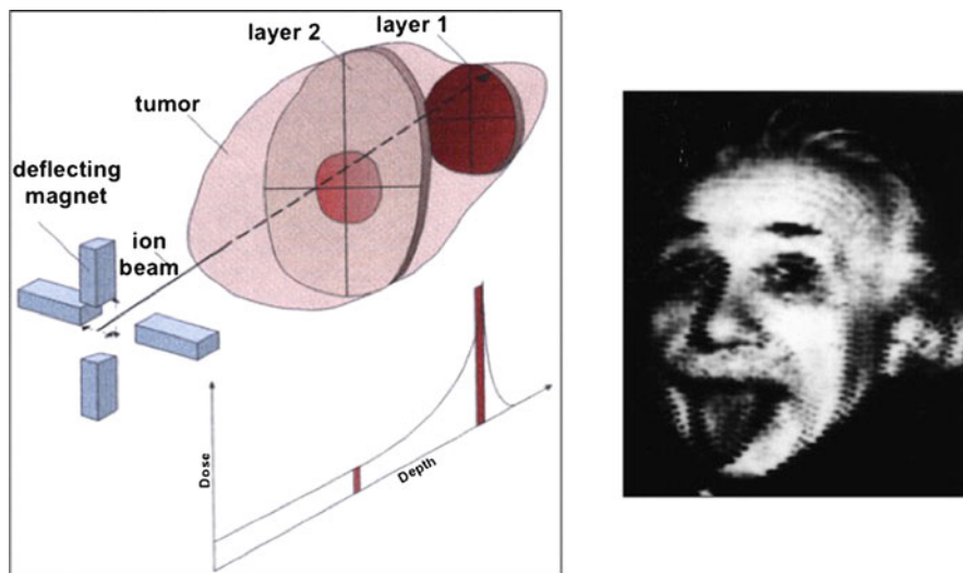
Fig. 4.6 Ion beam scanning. Left: Schematic view of the scanning technique. Individual slices of approx. 5 mm ( \approx Bragg peak width) are irradiated starting from the most distal part of the tumor and gradually moving forward. Within a slice the magnetically controlled ion beam is moved line-wise or from spot to spot to cover the desired target shape. The fact that proximal layers receive some dose (indicated by the dark central spot of layer 2) when more distal layers (1) are treated has to be taken into consideration by appropriately designing the irradiation protocol, e.g., give higher dose to the margin of layer 2 than to the preirradiated core. Right: Example of the raster scan capabilities: a pencil beam of carbon ions was used to reproduce a photo of Albert Einstein. Conditions were: 1.5 \times 10^{10} ions delivered in 80 fractions of 5 s each, beam diameter 1.7 mm FWHM, ion energy 480 MeV/u, photo plate 15 cm \times 18 cm. Data from GSI, Darmstadt, Germany
