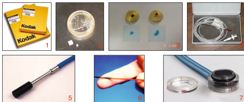
Fig. 26.2 Detectors for dosimetry: (1) Radiographic film for extended dose range (EDR-2), (2) Thermoluminescent dosimeter (TLD), (3) Gafchromic TM EBT (External Beam Therapy) film, (4) Hi-p silicon diode, (5) Tissue equivalent natural diamond, (6) Metal-oxide semiconductor field-effect transistor (MOSFET), (7) Plane parallel ion chamber Advanced Markus TM
