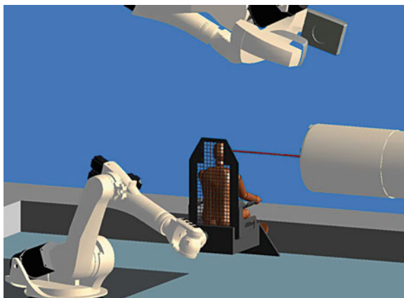
Fig. 33.12 Simulation of a treatment chair adapted to the robot positioner at a fixed beam. A patient can be rotated by 360^\circ allowing all treatment angles similar to a gantry
