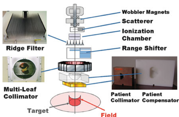
Fig. 37.2 Beam wobbling method with devices
