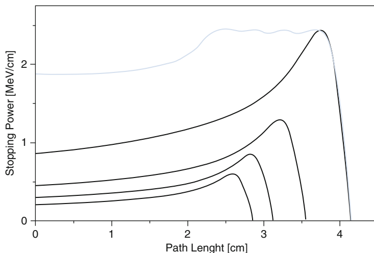
Fig. 25.4 Example how multiple Bragg peaks of different ranges can be added to approximate a flat spread-out depth dose distribution. The wiggles in the uppermost (blue) curve, which is the sum of the other curves, show that there are insufficient Bragg peaks used in this example to create a smoother SOBP for the desired SOBP width
