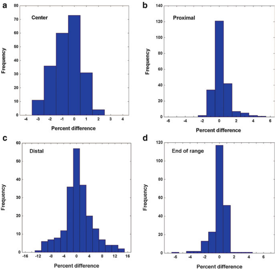
Fig. 28.3 Summary of all 2009 daily output data for Gantry 1. Measurements at the proximal and center points generally fall within \pm 2\% window. The measurements at the distal point are much broader, showing the challenges of point measurements in a rapidly changing dose gradient
