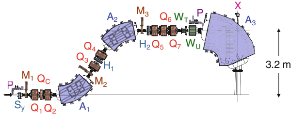
Fig. 24.2 Beam optics design of G2. The beam line consists of three main dipoles (A), seven quadrupoles (Q) three steering magnets (S), realized in combination with hexapoles (H), and pump (P) and beam profile monitors (M). The sweeper magnets WT and WU are controlled directly by the scanning system. The corrector quadrupole QC is wired in series to the U sweeper, in order to keep the beam well focused at the isocenter independently of scanning
