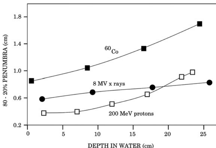
Fig. 6.1 Variation of the 80%–20% penumbrae as a function of depth for various radiation types
