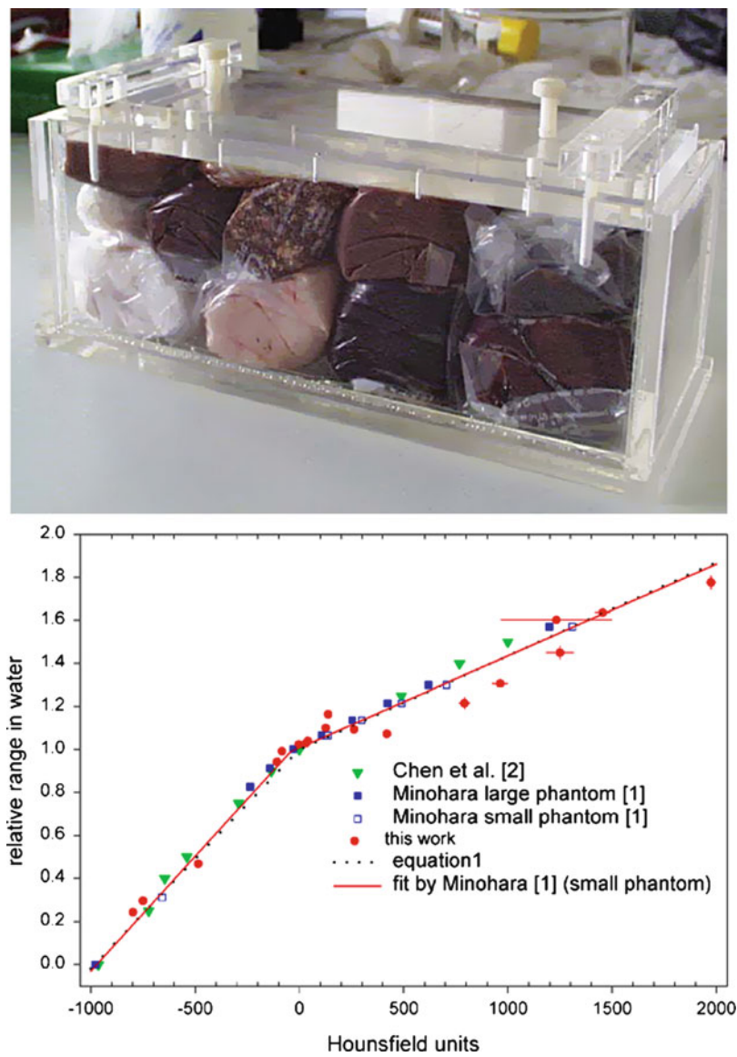
Fig. 29.2 Top: Typical phantom to validate the Hounsfield-to-range relation for ion beams as used, e.g., in [9]. It is composed of real animal tissue samples of different organs and put into a box of PMMA (polymethyl methacrylate), in order to have a well defined thickness for the range measurement. Bottom: Relation of the X-ray CT numbers to relative ranges of ions in water as derived from [8]. Several measured data sets are plotted together with a step-wise linear interpolation
