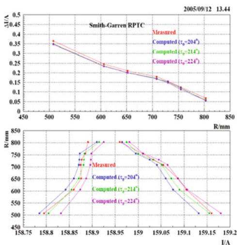
Fig. 23.9 Verification of isochronism conditions. Courtesy of Varian Medical Systems
