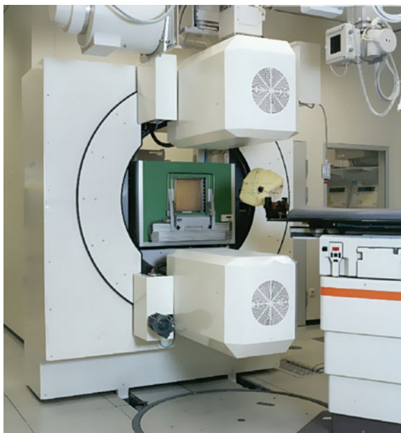
Fig. 31.4 The double-head positron camera at the GSI treatment site. The horizontal carbon ion beam leaves the beam pipe through a 20 \times 20 \text{ cm}^2 window visible in the center of the picture. To provide sufficient space for patient positioning, the PET scanner can be moved parallel to the beam between the measuring position (displayed) and the parking position [14]
