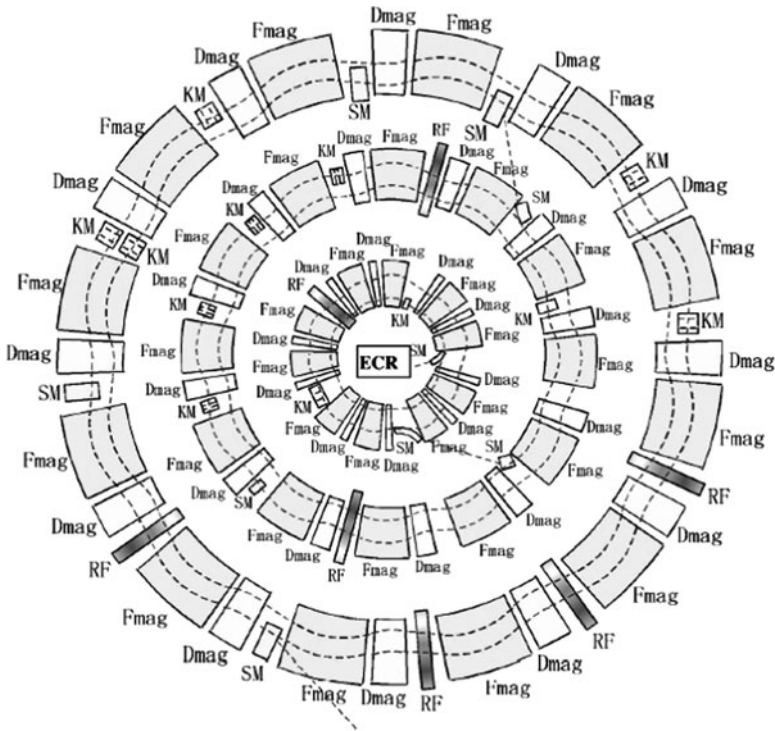
Fig. 20.5 Triple-cascade radial-sector FFAG accelerator [12]
