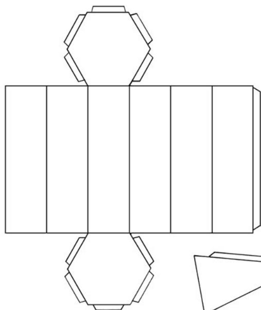
Hexagonal prism (10)
