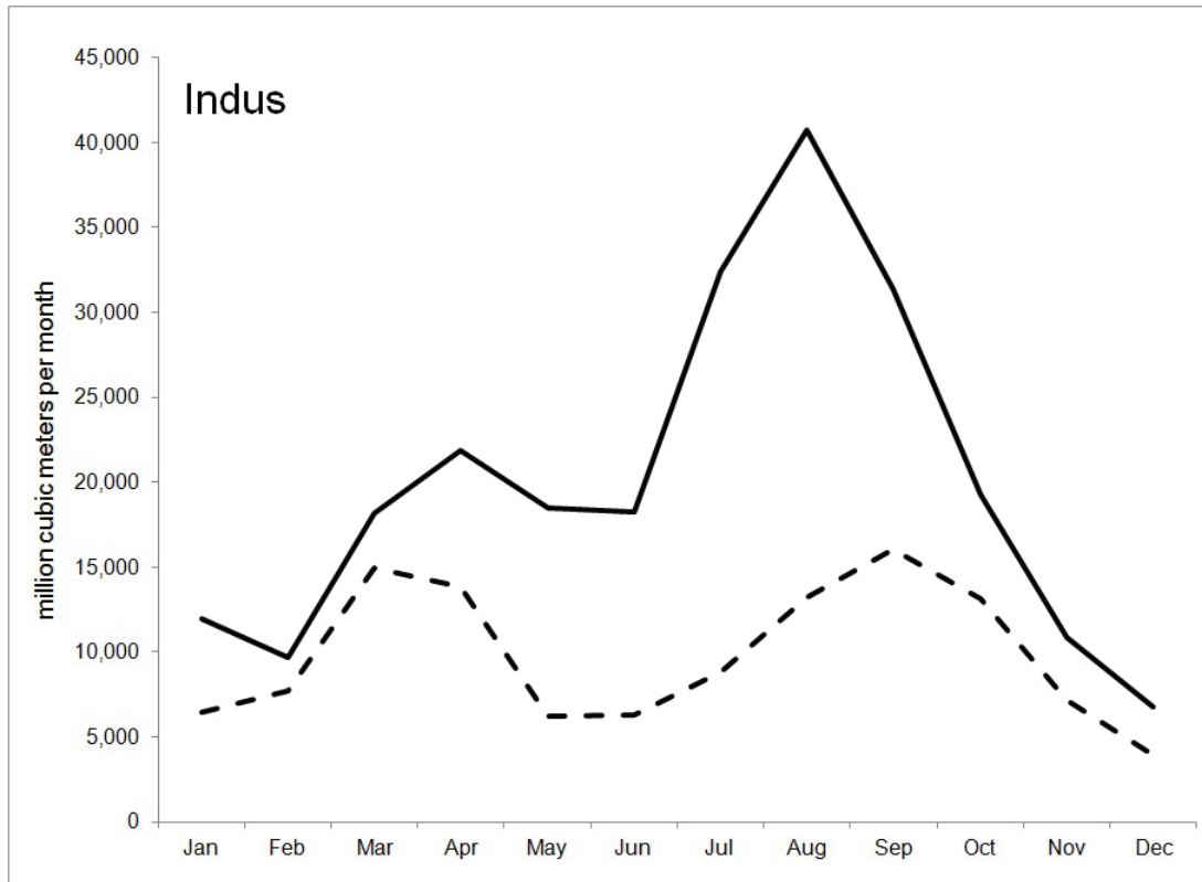
FIGURE 3.8 Natural run-off (solid line) and blue water consumed (dashed line) per month for the Indus. A higher percentage of the natural run-off is consumed than for the Ganges or the Brahmaputra basin, with the percentage highest in the period October to March. Water consumption does not exceed natural run-off in any month for the Indus. SOURCE: Based on data from Hoekstra and Mekonnen (2011).
