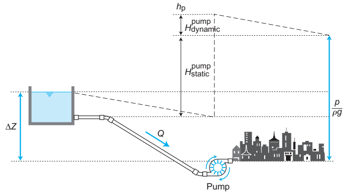
Figure 3.47. Booster stations.
