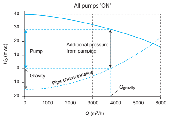
Figure A1.19. Pumping station operation – Problem A1.5.2b.
