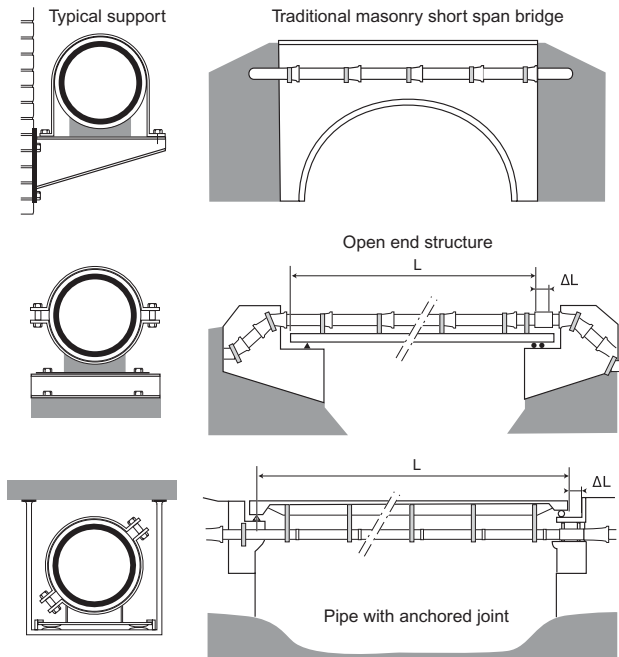
Figure 5.19. Pipe laying at a crossing (Pont-a-Mousson, 1992).
