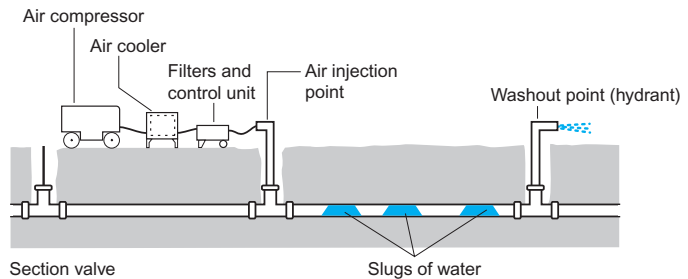
Figure 6.33. Air-scouring equipment and procedure.
