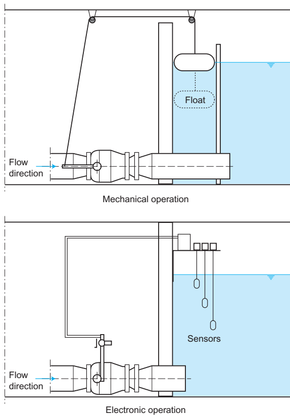
Figure 4.53. Operation of the float valve.
