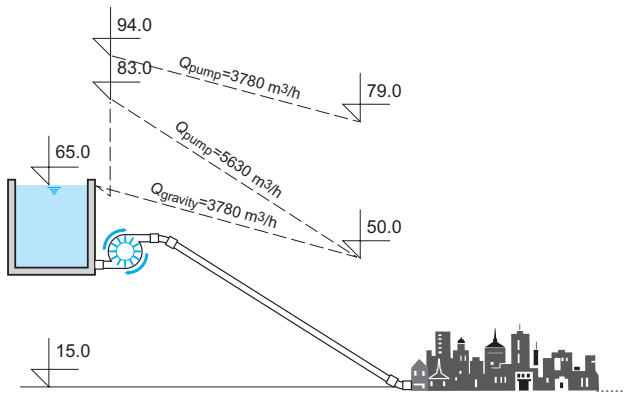
Figure A1.20. Hydraulic grade lines – Problem A1.5.2.
