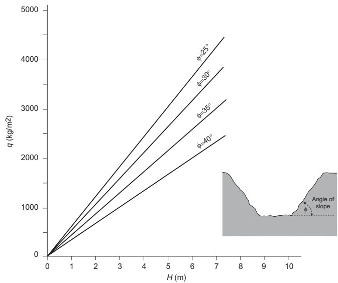
Figure 5.5. Trench slopes (Pont-a-Mousson, 1992).
