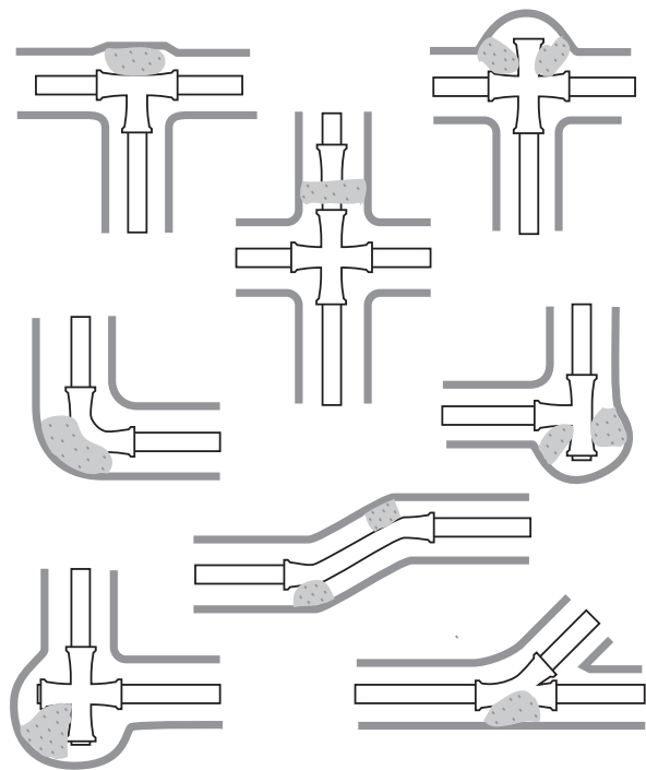
Figure 5.26. Thrust blocks in distribution systems (AWWA, 2003).
