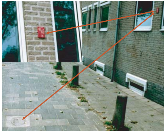
Figure 4.67. Locating underground hydrants (inset shows plate with coordinates).
