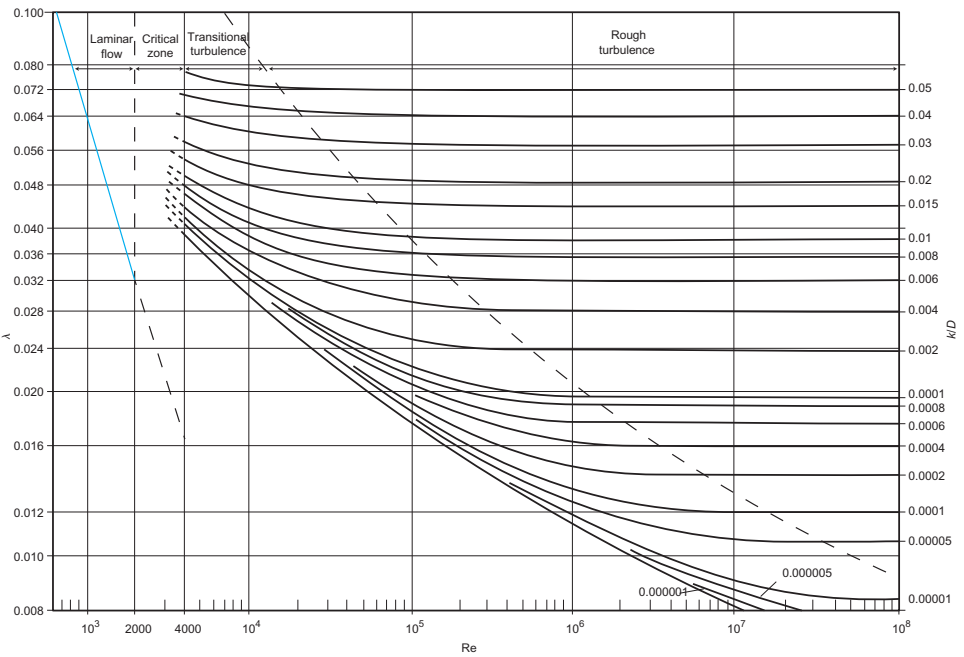
Figure 3.8. Moody diagram.
