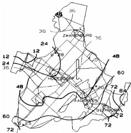
Figure 6.4. Retention times in a distribution network (Cohen and Konijnenberg, 1994).
