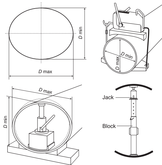
Figure 6.37. Correction of pipe deformation (Pont-a-Mousson, 1992).
