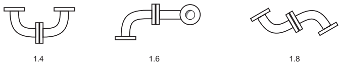
Figure A3.2. Multipliers for coupled 90°-bends.
