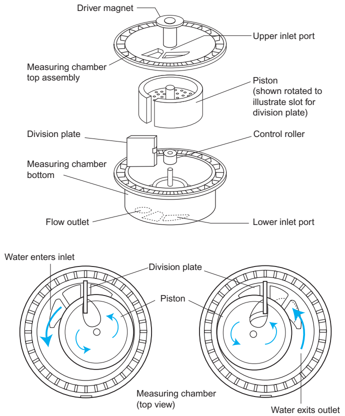
Figure 4.63. Principle for operation of the rotary piston.
