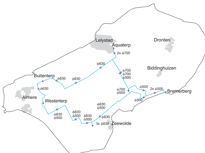
Figure 4.4. Looped water transport system (Province of Flevoland, 1996).
