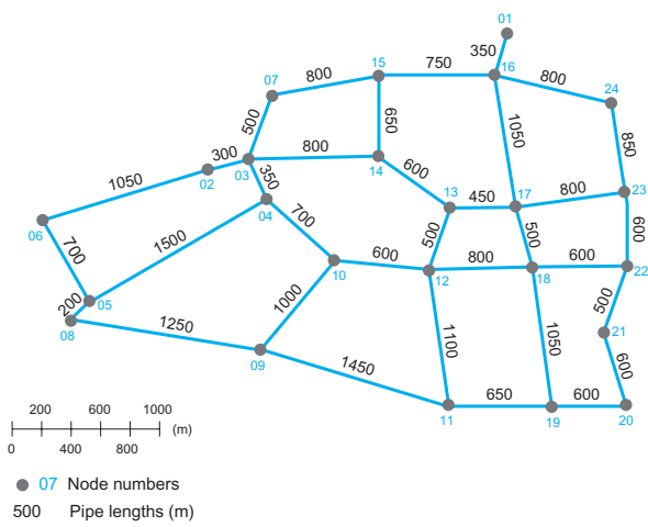
Figure A2.3. Node numbers and pipe routes.
