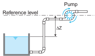
Figure 4.21. Pump unit located above the suction level in the reservoir.
