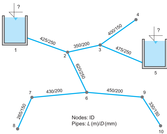
Figure A1.3. Network layout – Problem A1.3.2.
