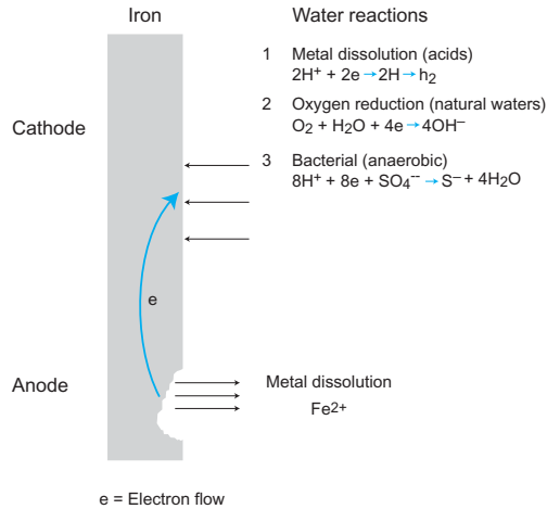
Figure 6.27. Metallic corrosion.
