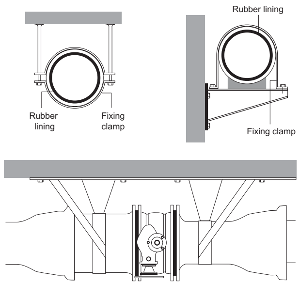
Figure 5.20. Pipe laying when crossing a road (Pont-a-Mousson, 1992).
