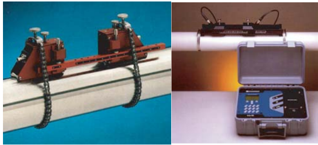
Figure 4.60. Ultrasonic meters (Manufacturers: Controlotron – left and Dynasonic – right).
