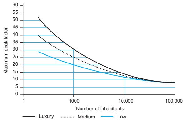
Figure 2.8. Simultaneity diagram of various categories of accommodation.
