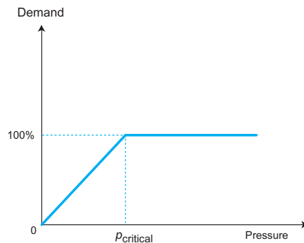
Figure 3.23. Pressure-related demand relation (KIWA, 1993).
