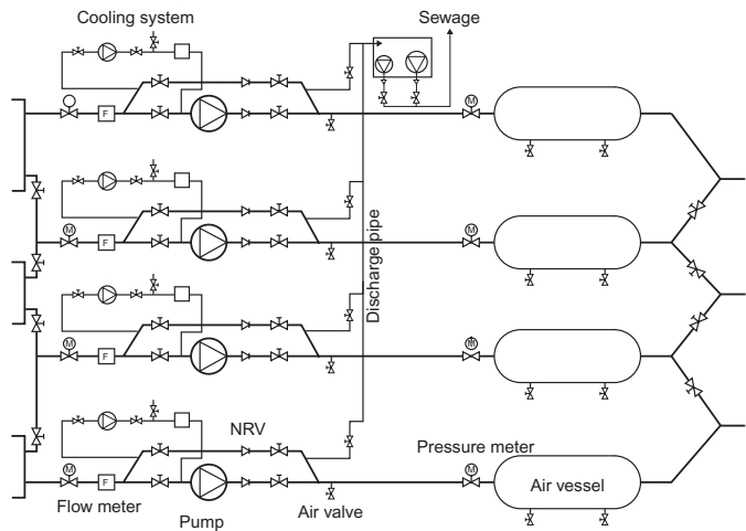
Figure 4.17. Pumping station layout.
