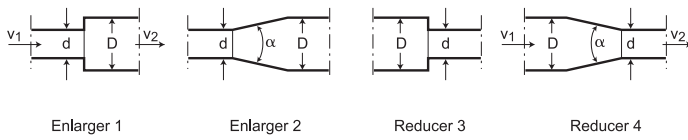
Figure A3.4. Geometry of pipe enlargements and reducers (Table A3.3).
