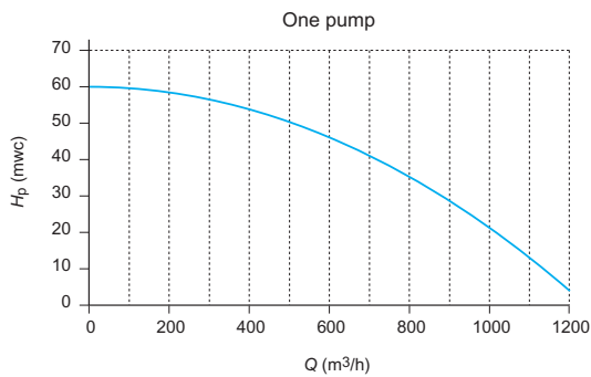
Figure A1.27. Pump characteristics – Problem A1.5.6.
