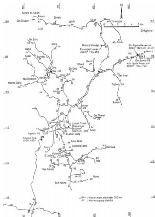
Figure 4.3. Branched water transport system in Palestine (Abu-Thaher, 1998).
