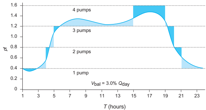
Figure 4.11. Balancing volume in the case of scheduled pumping.
