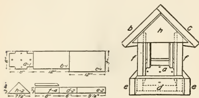
FIGURE 156.—PLAN FOR BIRD HOUSE.
